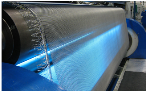
Stainless steel mesh is cut, pre-treated, and powder coated
