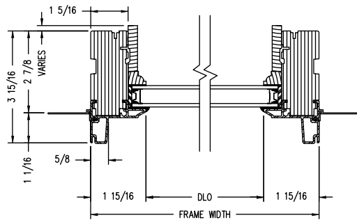
Horizontal Section
