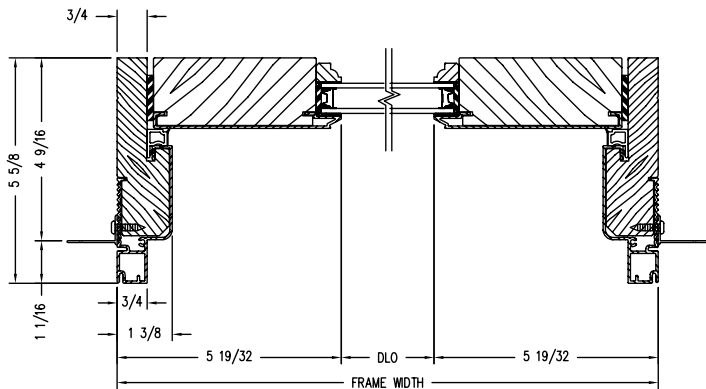
Horizontal Section
