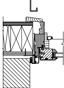
Expander Return
