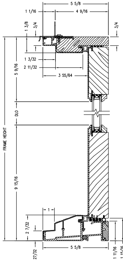
(Drainage Sill)
