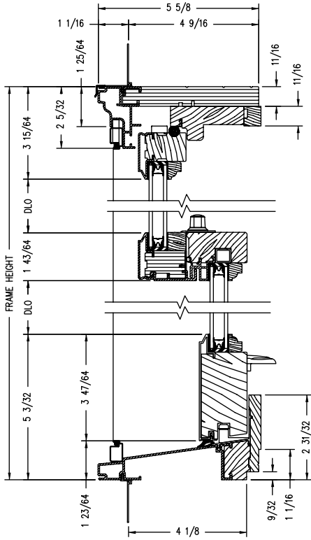
Vertical Section
