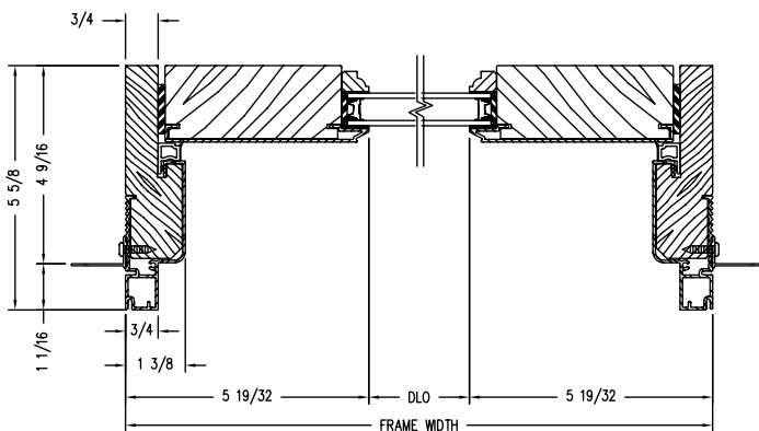
Horizontal Section
