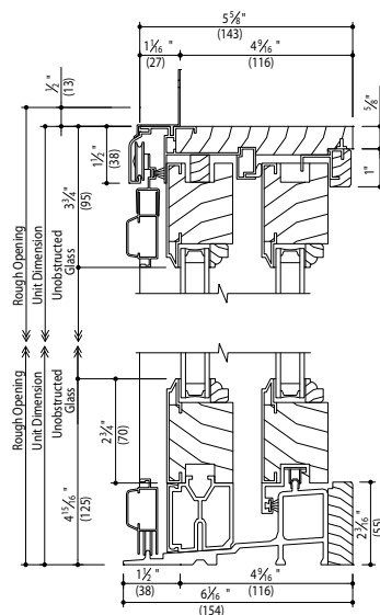
Vertical Section
