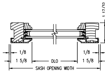
Horizontal Section
