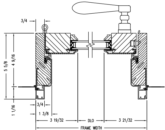
Horizontal Section
