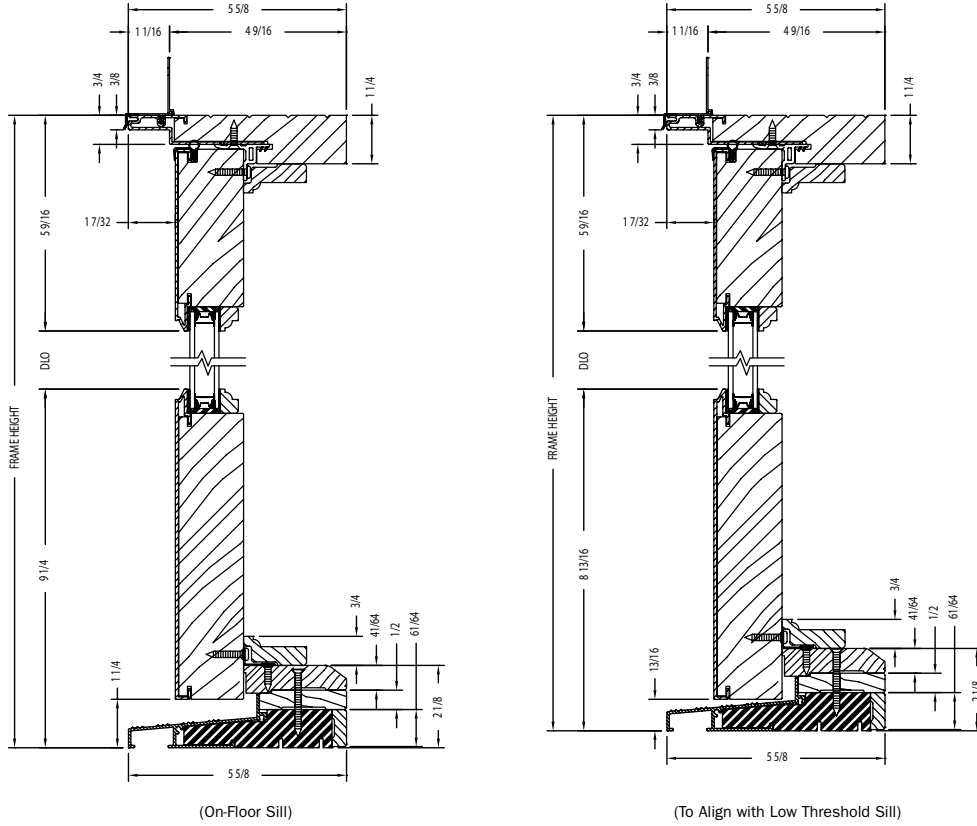
Vertical Section
