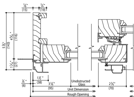
Horizontal Section
