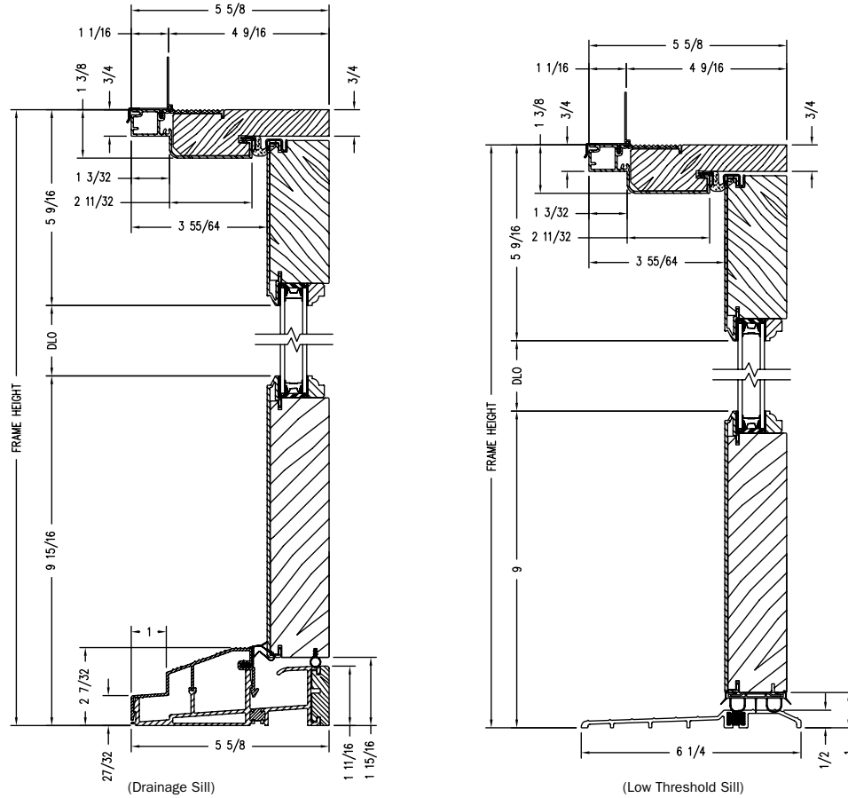
Vertical Section
