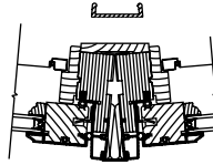
10° Casement Bow Exterior Mull Cover
