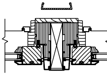
1" Exterior Mull Cover
