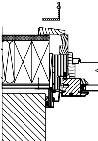
3/4" Frame Enclosure
