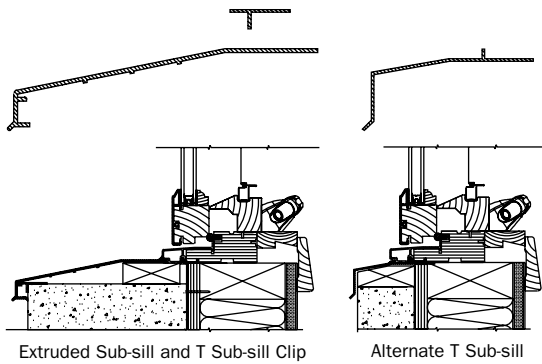
Extruded Sub-sill and T Sub-sill Clip
