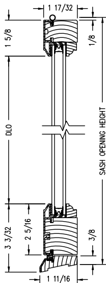
Vertical Section
