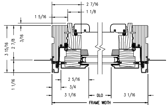
Horizontal Section
