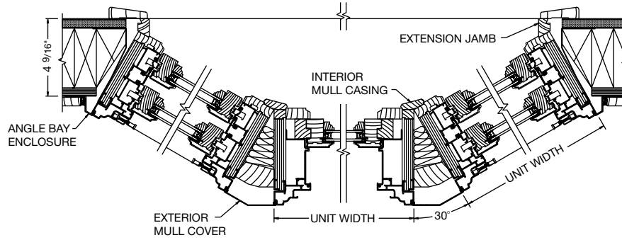
Horizontal Section
