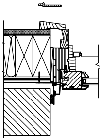
3/4" Frame Extender
