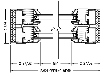
Horizontal Section
