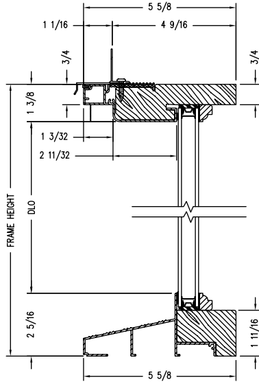
Vertical Section
