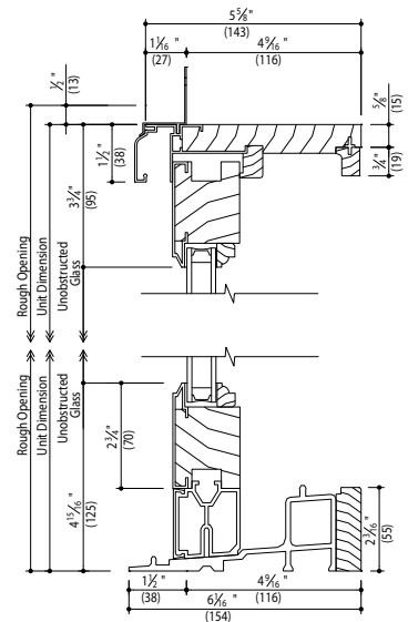
Vertical Section
