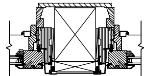
1" - 5" Adjustable Mull Cover and Receiver (vertical join)
