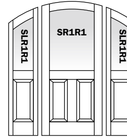
2 3/8" stiles, 4 1/16" stiles, 4 1/16" top rail, 4 1/16" top rail, 8" bottom rail 8" bottom rail & raised panel insert & raised panel insert
