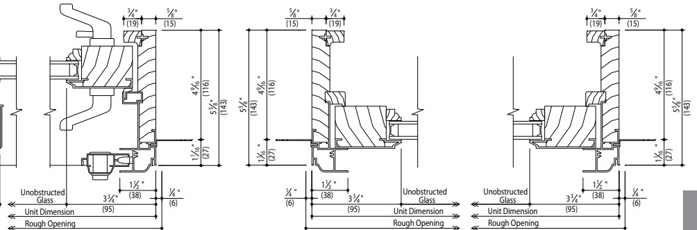
Horizontal Section
