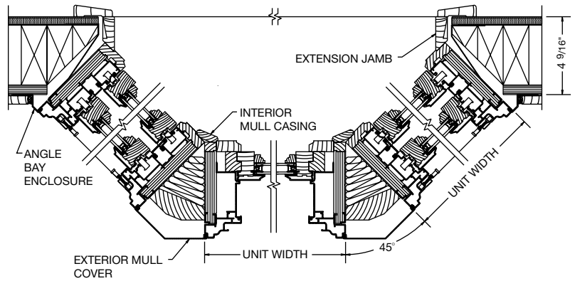
Horizontal Section
