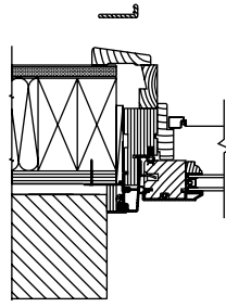
3/4" Frame Expander
