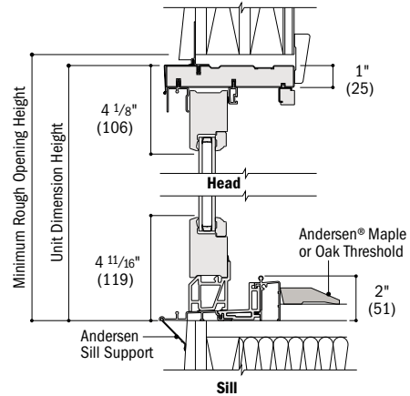
Vertical Section Stationary
