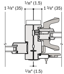
Perma-Shield® Gliding to Perma-Shield® Gliding
