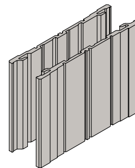
¾" (19) x 7 ¾" (197) Fiberglass Joining Material For higher performance for 1-way and 2-way joining. Required for hinged inswing patio doors with 6 7/16" (167) or greater exterior extension jamb depths.
