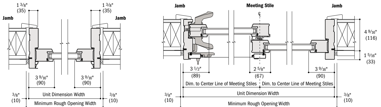
Horizontal Section Stationary
