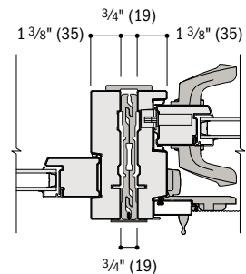
Perma-Shield® Gliding to Perma-Shield® Gliding
