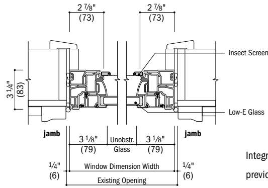
Horizontal Section Existing Window Opening
