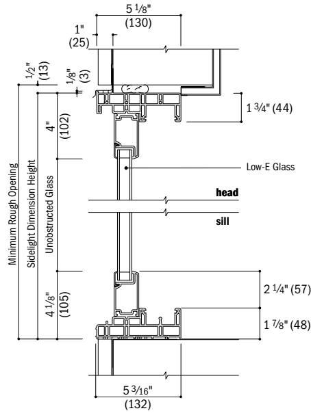
Vertical Section Sidelight, Stucco Exterior
