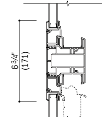
Vertical Section Transom Over Single-Hung
