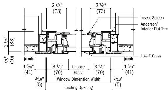
Horizontal Section Existing Aluminum Frame Window Opening
