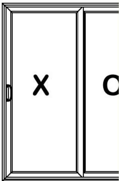
C774 - Double Slider
